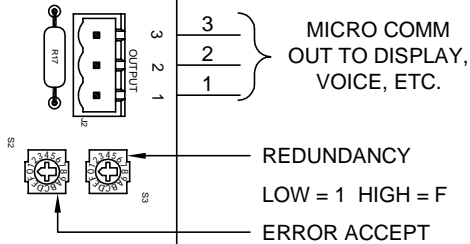
TYPICAL MICRO COMM CONNECTOR 1=COM 2=V+ 3=DATA
