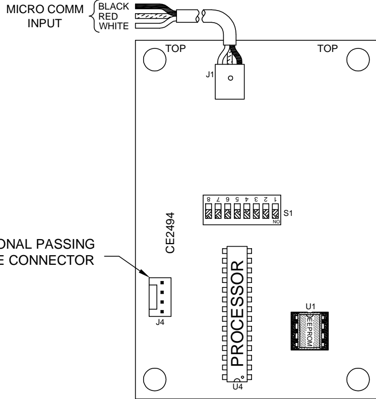
CE2494 DRIVER BOARD
