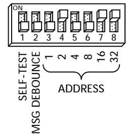
DIP SWITCH DETAIL
