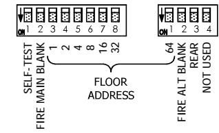
S1 - DIP SWITCH DETAIL - S2
